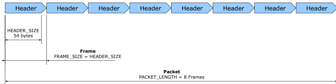
Figure 5.2: Data organization in Header and Packets in „StoreDisabled“ mode
